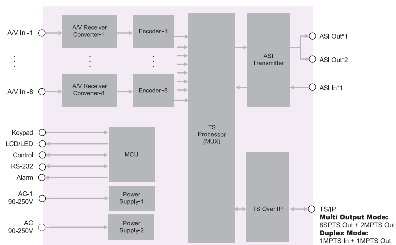
NKP-4800/4801EC Functional Block Diagram
